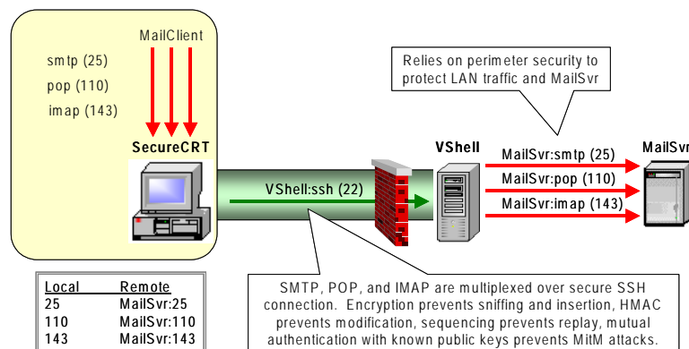
Figure 2: Local Port-forwarding
